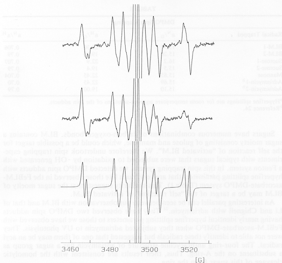
FIGURE 1 EPR Spin Trapping. Top and middle spectra are consecutive 80 gauss/11.2 min scans of an EPR spin trapping experiment in which 30 \mu\text{M} BLM that had been preincubated with 10 \mu\text{M} Fe(III) was introduced to a phosphate-buffered, pH 7.4, 500 \mu\text{M} ascorbate solution containing 50 \text{ mM} DMPO. Receiver gain, 2 \times 10^6 ; microwave power, 40 \text{ mW} ; modulation amplitude, 1.0 \text{ G} . These spectra were simulated (bottom spectrum) assuming the presence of three distinct species; two DMPO spin adducts and the ascorbate free radical (the strong ascorbate radical signal is the off-scale center doublet). The parameters used for this simulation were: DMPO/adduct 1- a^{\text{N}}_1 = 15.75 \text{ G} , a^{\text{H}}_1 = 22.30 \text{ G} , \Delta\text{Hpp} = 1.60 \text{ G} ; for DMPO/adduct 2- a^{\text{N}}_2 = 15.20 \text{ G} , a^{\text{H}}_2 = 19.20 \text{ G} , \Delta\text{Hpp} = 2.0 \text{ G} , \Delta g = -0.2 \text{ G} ; the ascorbate radical; a^{\text{H}} = 1.8 \text{ G} , \Delta\text{Hpp} = 1.0 \text{ G} , \Delta g = 0 \text{ G} . Only the ascorbate radical is observed in the absence of BLM or DMPO. If BLM is omitted, only a weak ascorbate radical signal is observed. An oxygen-containing, near-neutral solution of ascorbate will have a very low level of the ascorbate radical present, even in the absence of significant adventitious metals. 16 This low level of \text{Asc}^{\cdot -} is thought to arise from the autoxidation of the dianion of ascorbic acid. 13,16
