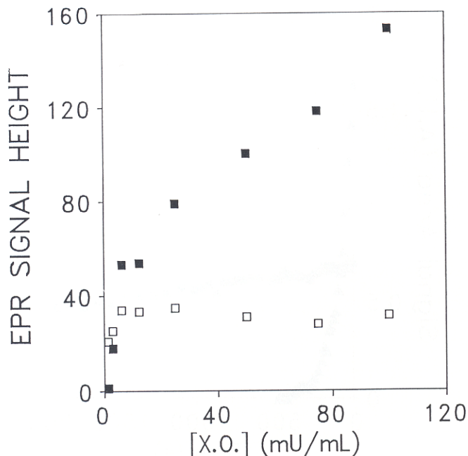
FIGURE 3 Relative EPR signal intensity of DMPO/·OOH (■) and DMPO/·OH (□) as the concentration of xanthine oxidase is varied in a HX/X.O. superoxide-generating system.
