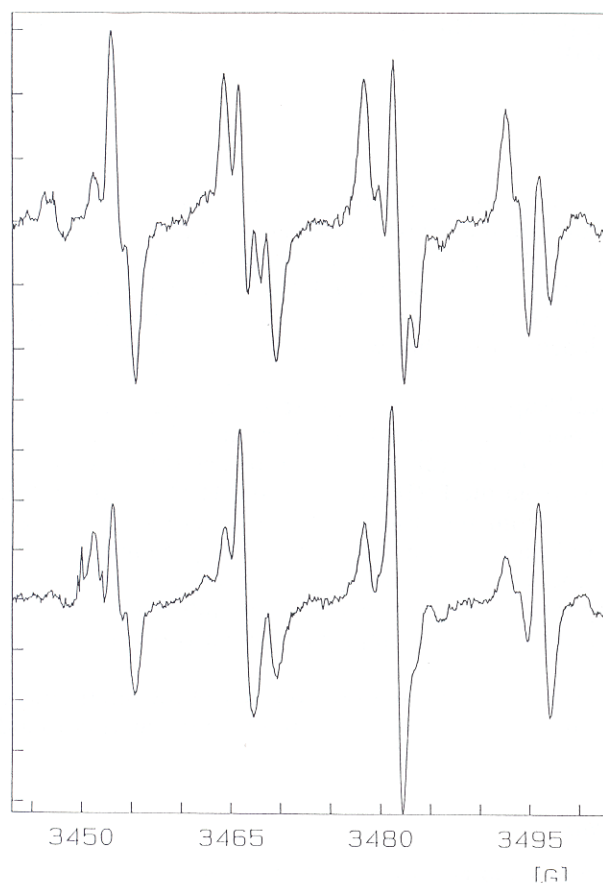
FIGURE 6 EPR spectra of DMPO/ \cdot OOH and DMPO/ \cdot OH. These samples were generated outside the cavity with the riboflavin/DETAPAC and light system. Within 5 s after cessation of illumination, the sample was drawn into a flat cell in the cavity and spectral scans were initiated. Top : No added iron. Bottom : 20 \mu M Fe(II) added immediately after cessation of illumination. Instrument settings: 0.95 G mod. amp.; 5 \times 10^5 receiver gain; 40 mW power; time constant 0.17 s; scan 60 G/84 s. With this scan rate, there is 55 s between the high and low field lines of DMPO/ \cdot OOH.
