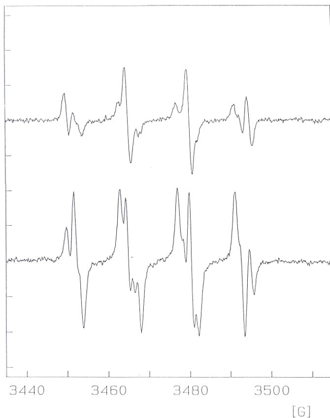
FIGURE 4 EPR spectra of DMPO/·OOH generated by the HX/X.O. system. Upper spectrum: The system contained: 50 mM DMPO; 0.5 mM hypoxanthine; 50 \mu M DETAPAC; and xanthine oxidase, \approx 3 mU/mL in 50 mM pH 7.8 phosphate buffer. Bottom spectrum: All ingredients were the same except that xanthine oxidase was present at \approx 25 mU/mL. Instrument settings were: 40 mW microwave power; 0.96 gauss modulation amplitude; 0.33 s time constant; 80 gauss/168 s scan rate; receiver gain, 1 \times 10^6 top, 5 \times 10^5 bottom. The EPR scan was initiated \approx 3.5 minutes after the introduction of X.O.
