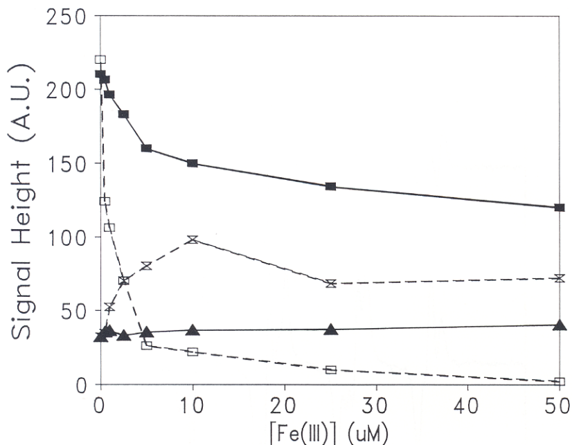
FIGURE 5 Relative intensity of DMPO/·OOH (■ and □) and DMPO/·OH (▲ and X) in a pH 7.4 phosphate buffer solution that contains 1 mM HX, 25 mU/mL X.O., 50 mM DMPO, 250 μM EDTA (dashed lines) or 250 μM DETAPAC (solid lines), and varying concentrations of Fe(III).
