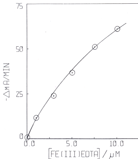
FIGURE 1 This curve was obtained in 50 mM demetallated phosphate buffer pH 7.40 containing 50 \mu\text{M} EDTA and 125 \mu\text{M} ascorbate (265 nm absorbance, 1 cm, at time zero = 1.8). mA = milliabsorbance units
