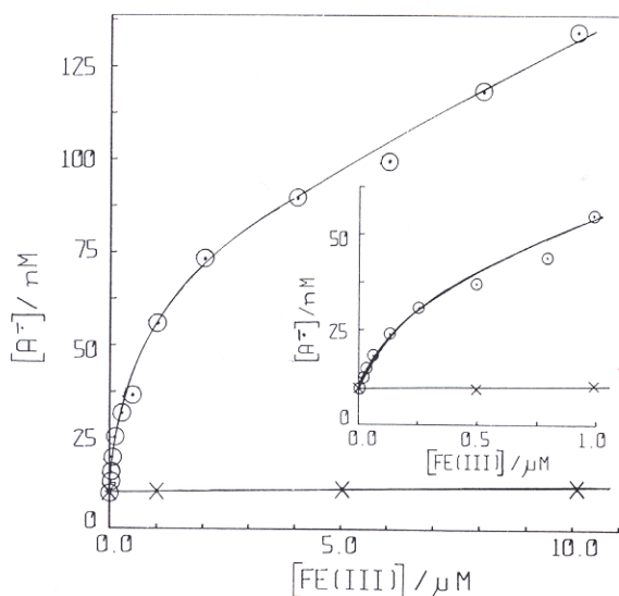
FIGURE 2 These curves were obtained in 50\ \text{mM} demetalled phosphate buffer pH 7.40 containing 250\ \mu\text{M} ascorbate and 250\ \mu\text{M} EDTA (O) or 50\ \mu\text{M} Desferal (X).
